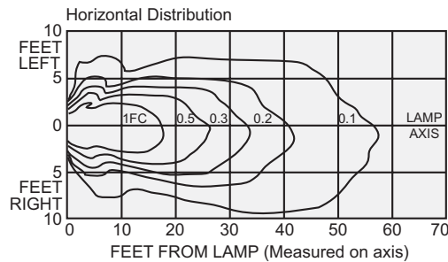
6V, 9W Tungsten Wedge Base Lamp (ANSI 908), Round Head (Replacement Lamp NL6V9WB)
